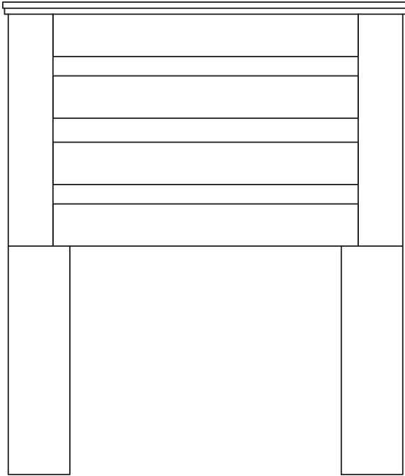
Wittenberg Headboard Twin WN42T 42"W x 2"D x 47"H Full WN56F 56"W x 2"D x 47"H Queen WN62Q 62"W x 2"D x 47"H
