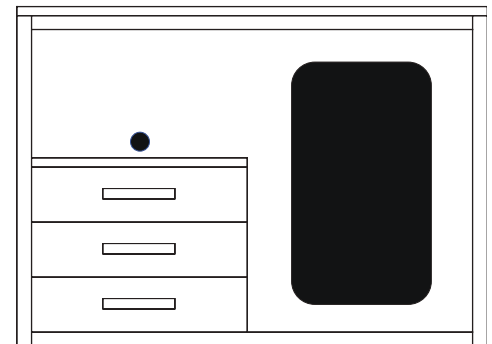
Sullivan Micro Fridge - 3 Drawer SUL48MF 48'W x 24'D x 37'H
