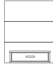
Wall Mount Night Stand (Drawer) ITEM# LD18D 18"W x 16"D x 7"H
