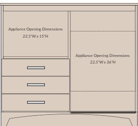
NODA Micro-Fridge Unit - NO Trim Available upon Request 48'W x 22'D x 43'H
