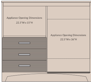
DECO Espresso Micro Fridge Unit - NO Trim ITEM# Available upon Request 48"W x 22"D x 43"H DECO Espresso Micro Fridge Unit with Metal Trim Shelf Protection ITEM# DC16MF 48"W x 22"D x 43"H
