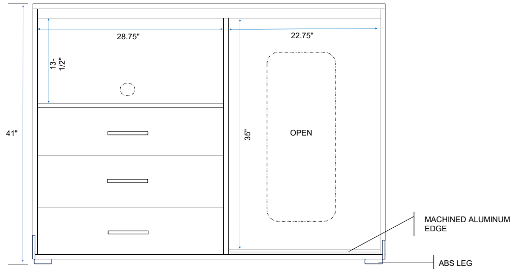
FRONT VIEW
