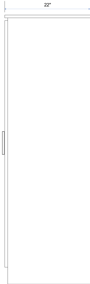
SIDE VIEW
